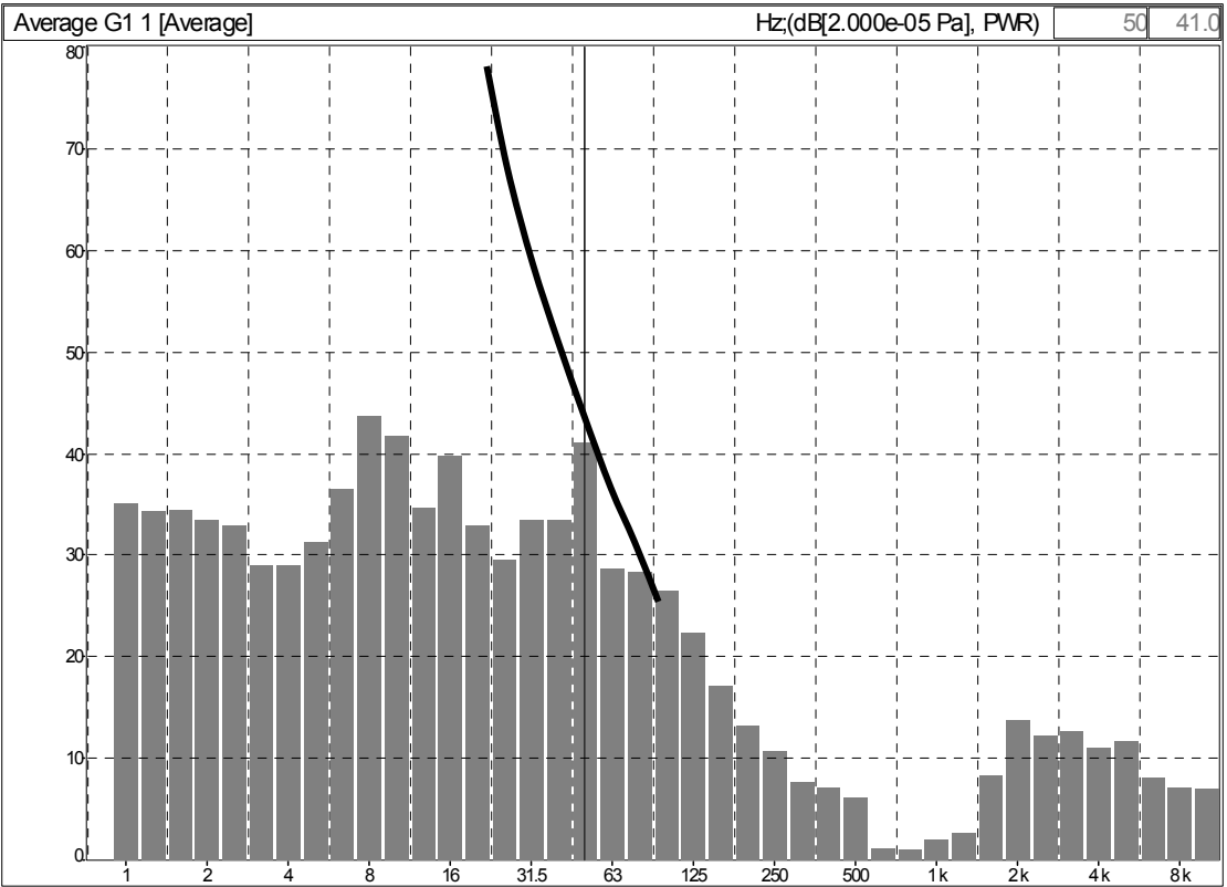
Figure 84: Mean 1/3 octave band spectrum starting 05h10m on 25/04/04 from measurement Case18_040424_205000.cmg
