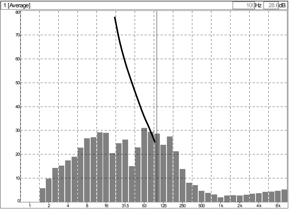
Figure 77: Mean 1/3 octave band spectrum during 2m10s of flyover starting at 02h33 on 06/04/04 from measurement Case16_040405_210000.cmg
