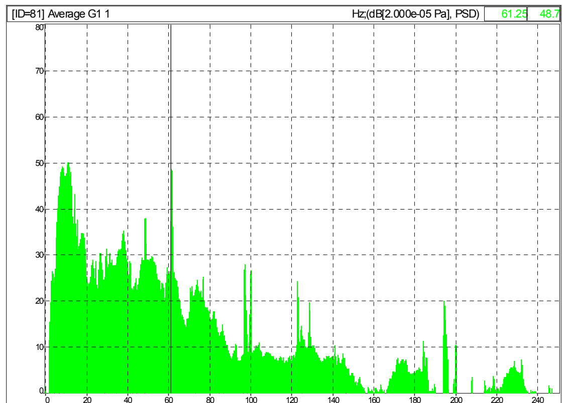
Figure 96: FFT of 9m30s audio record starting 07h00m from measurement Case19a_040424_090000.cmng
