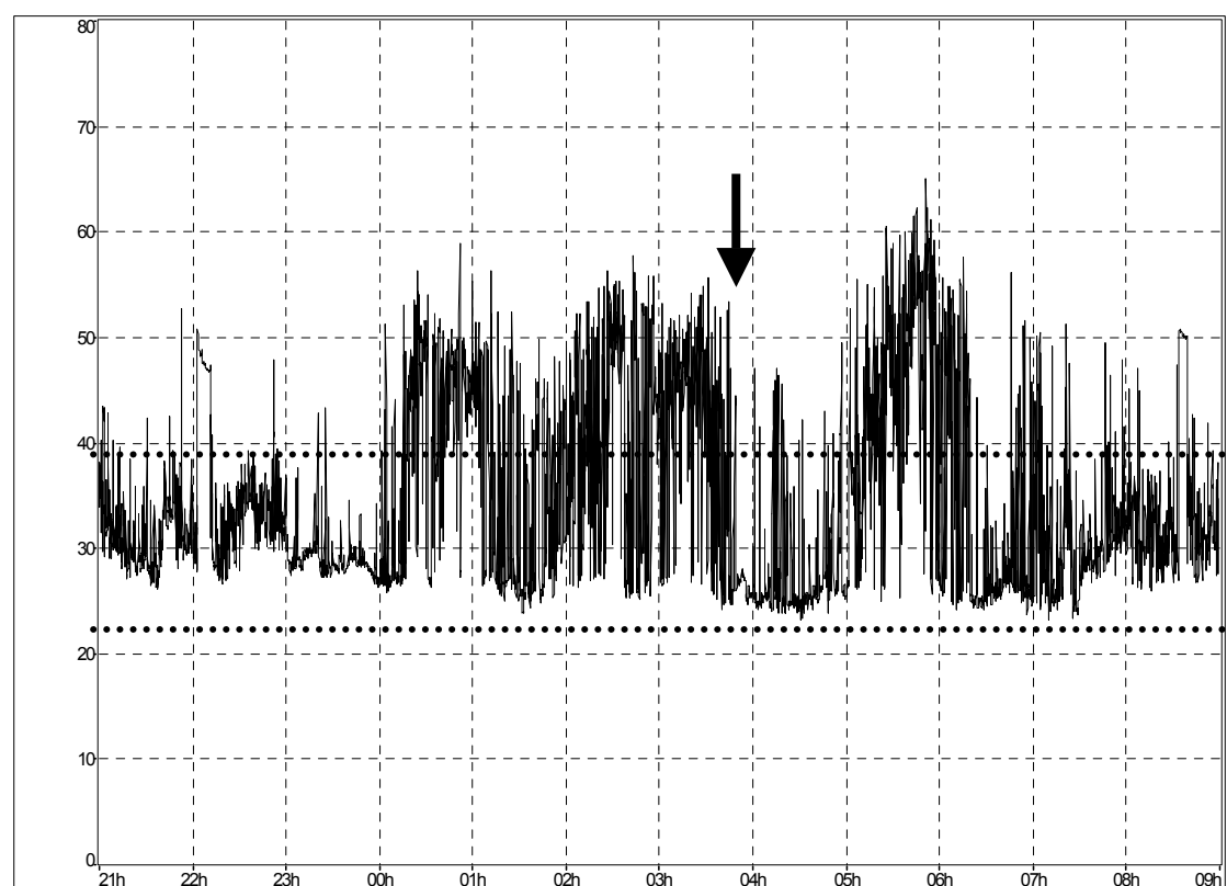
Figure 49: Time history showing 100Hz 1/3 octave spectrum band from measurement Case6_040513_210000.cmg together with Dutch (audibility) 22dB and Danish 39.1dB limits
