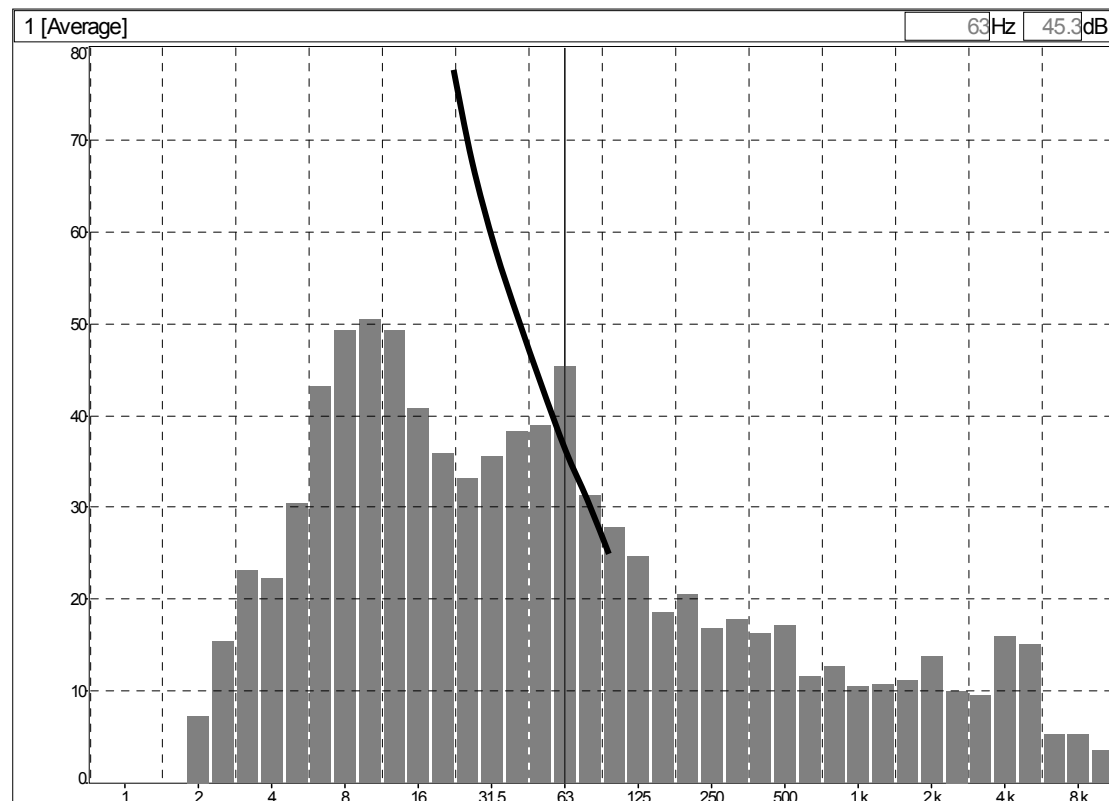
Figure 97: Mean 1/3 octave band spectrum 9m30s starting 07h00m from measurement Case19a_040424_090000.cmg
