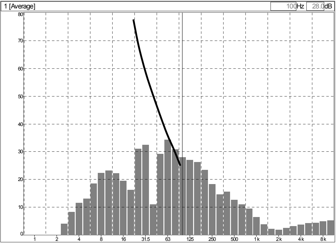
Figure 73: Mean 1/3 octave band spectrum of 3m00s starting 04h10m on 03/04/04 from measurement Case16_040402_210000.cmg
