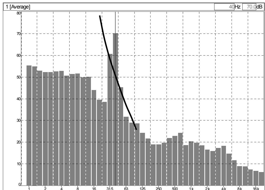
Figure 4: Mean 1/3 octave band spectrum 9m30s starting 03h00m from measurement Case20_458_210000.cmg
