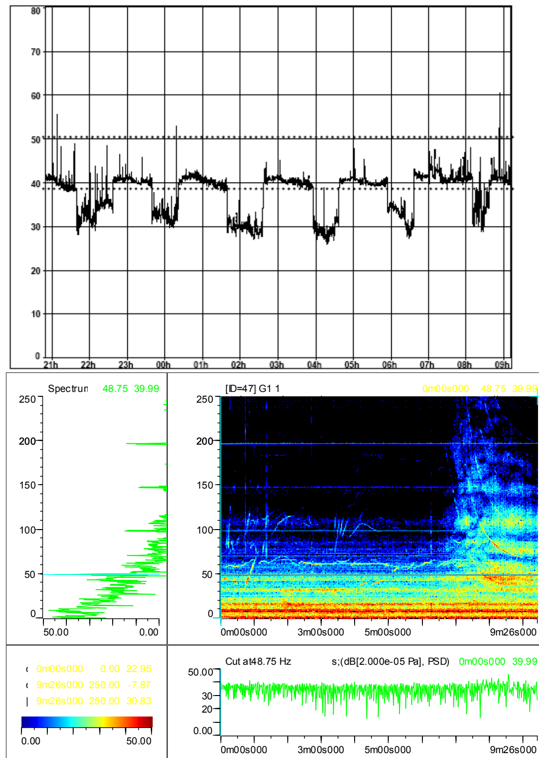
Figure 86: Sonogram of 9m30s of audio record starting 05h10m on 25/04/04 from measurement Case18_040424_205000.cmg. Illustrating falling tones varying in frequency for example from 200 to 40Hz. Constant tone at ~50Hz is due to the fridges with harmonics at 100, 150 and 200Hz.
